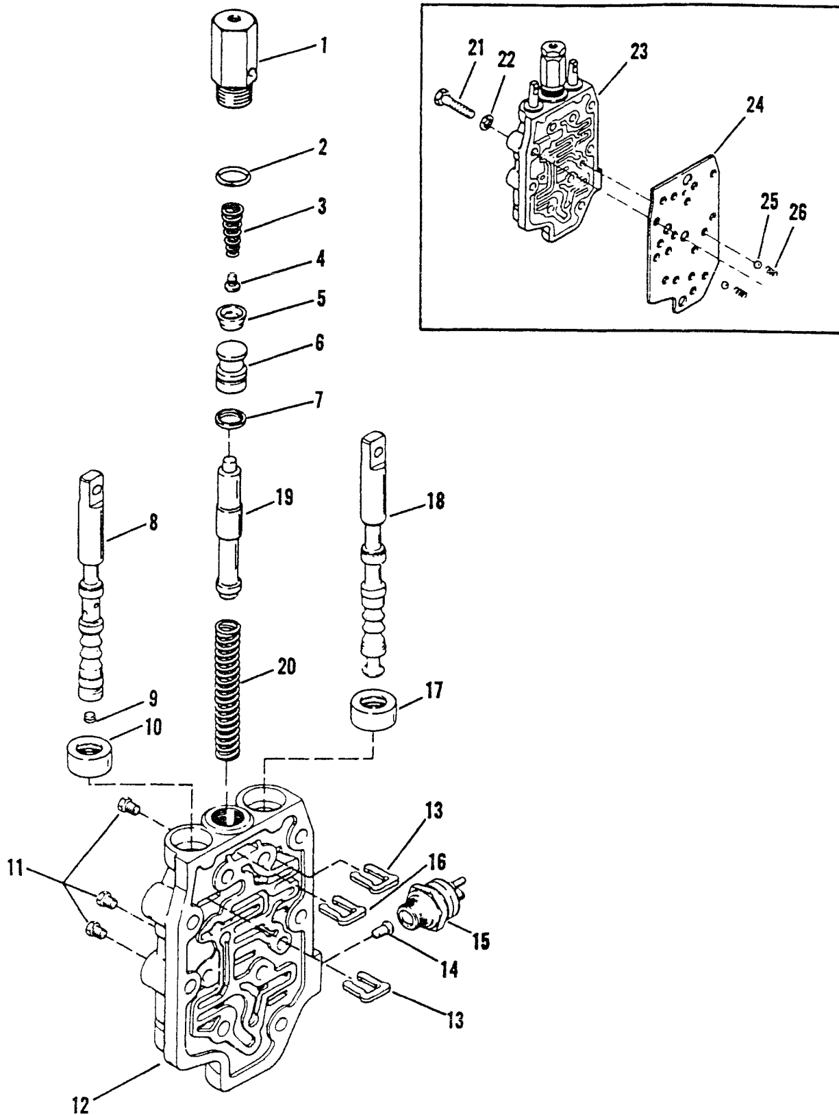
HYDRAULIC DECLUTCH
