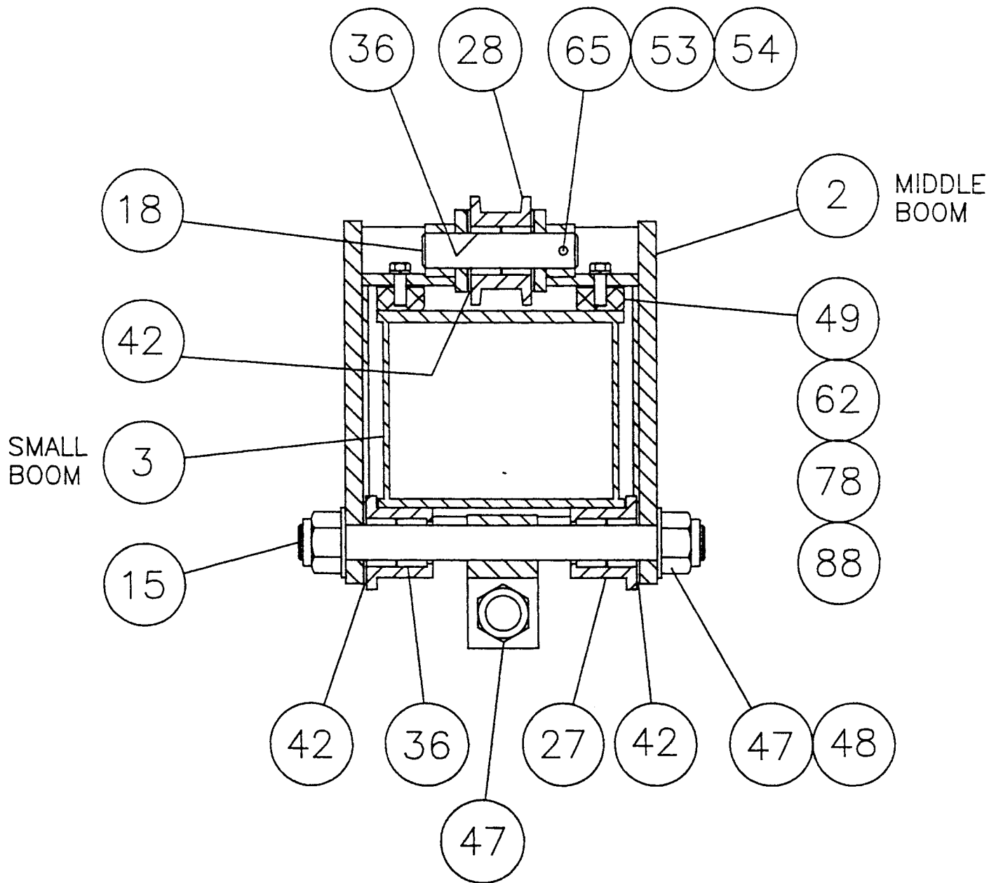
VIEW OF FRONT ROLLERS SUPPORTING SMALL BOOM
